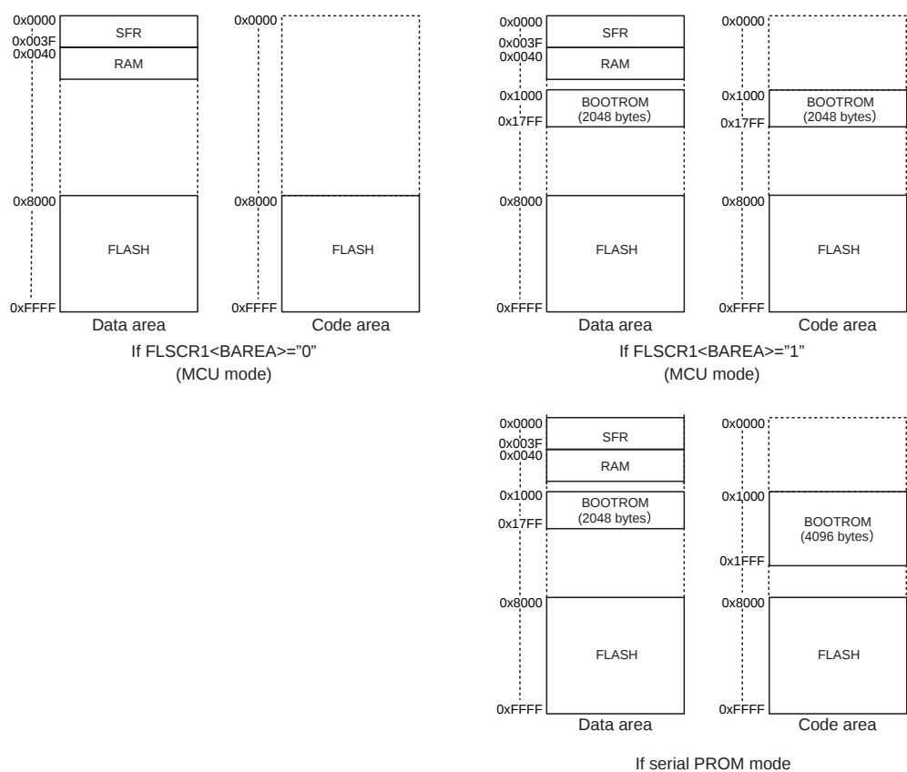
Figure 22-3 Memory Mapping
