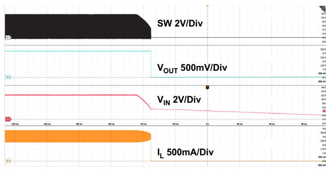
Figure 26. Shutdown through V_{\text{IN}} ( I_{\text{OUT}} = 3\text{A} )
