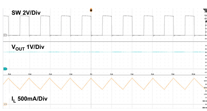
Figure 15. Steady-State Operation, I_{OUT} = 3\text{A} ( V_{OUT} = 5\text{V} )
