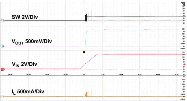
Figure 23. Startup through V_{\text{IN}} ( I_{\text{OUT}} = 0\text{A} )
