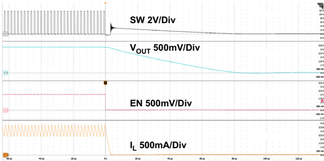
Figure 30. Shutdown through EN ( I_{OUT} = 3\text{A} )
