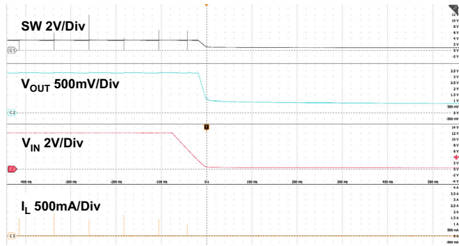
Figure 24. Shutdown through V_{\text{IN}} ( I_{\text{OUT}} = 0\text{A} )
