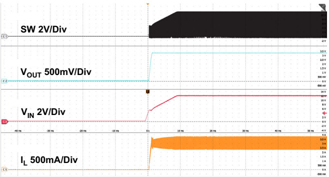
Figure 25. Startup through V_{\text{IN}} ( I_{\text{OUT}} = 3\text{A} )
