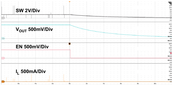
Figure 28. Shutdown through EN ( I_{OUT} = 0\text{A} )
