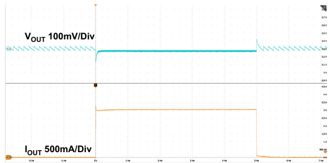
Figure 39. Load Transient, 0A to 3A (0.5A/μs)
