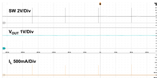
Figure 11. Steady-State Operation, I_{OUT} = 0\text{A} ( V_{OUT} = 5\text{V} )
