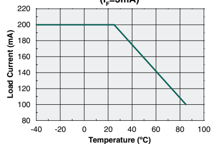
Maximum Load Current vs. Temperature ( I_F=3\text{mA} )
