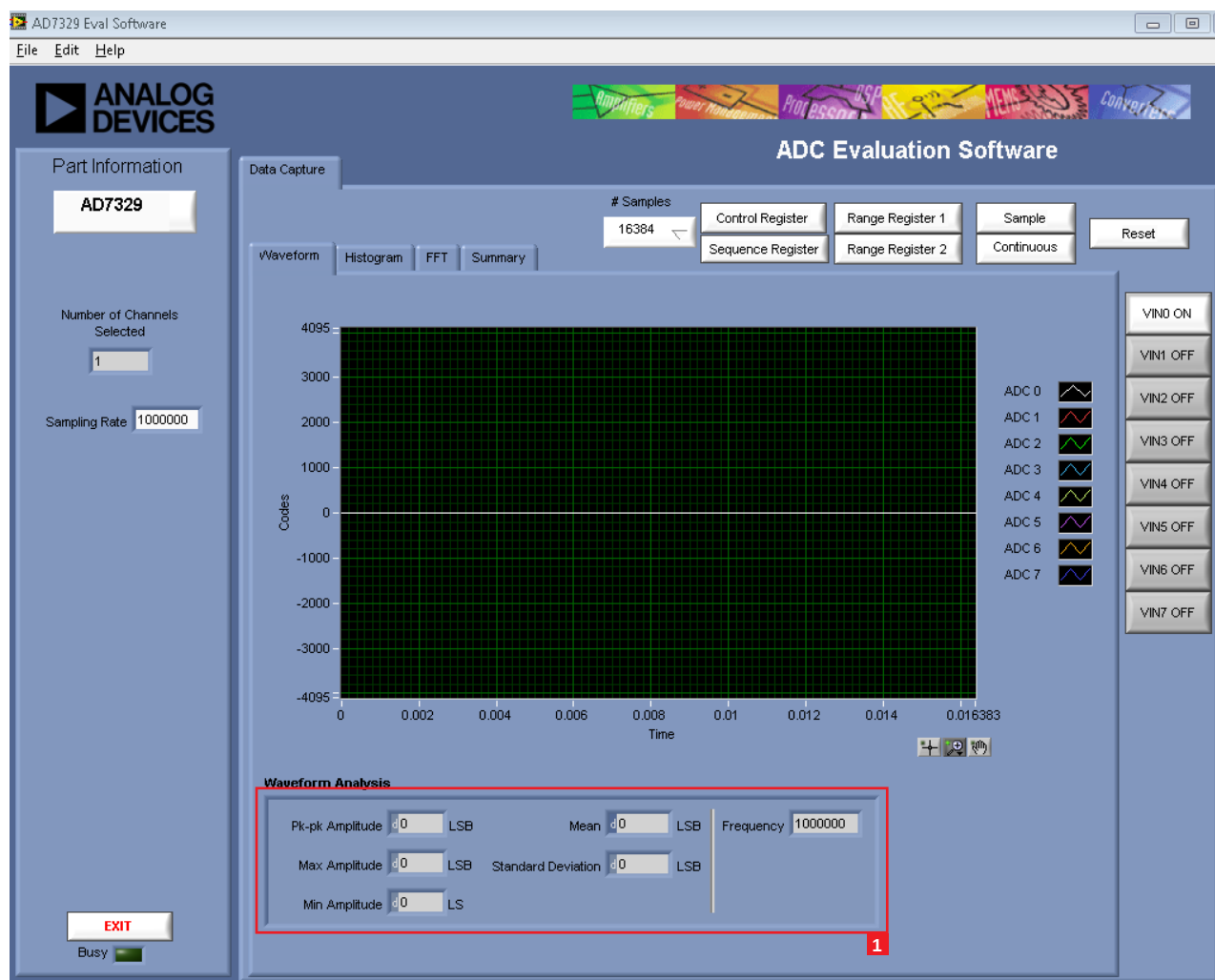
Figure 22. Waveform Tab
