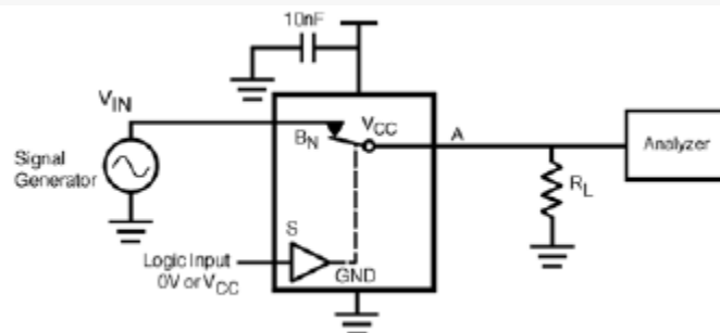
Figure 14. Harmonic Distortion
