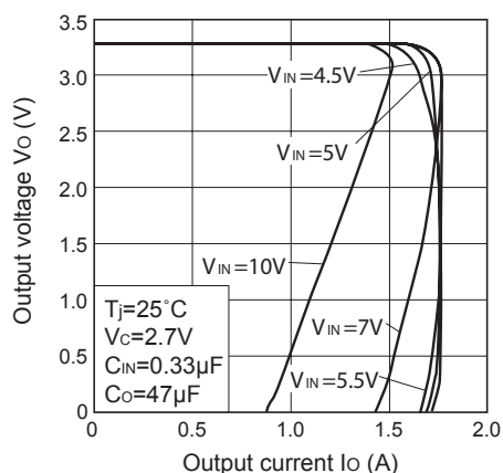
Fig.7 Overcurrent Protection Characteristics (Typical Value, PQ033EF01SZH)
