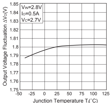
Fig.9 Output Voltage Fluctuation vs. Junction Temperature (PQ018EF01SZH)
