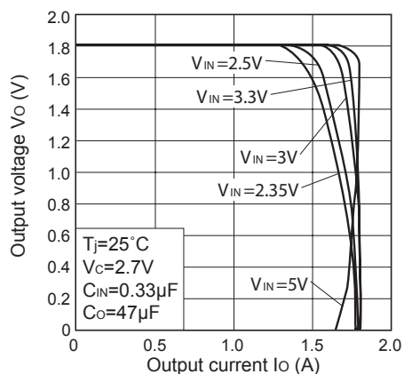
Fig.5 Overcurrent Protection Characteristics (Typical Value, PQ018EF01SZH)
