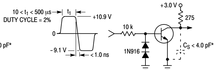
Figure 3. Turn-Off Time
