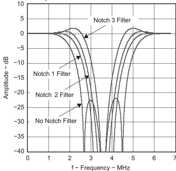
Figure 2-6. Chroma Trap Filter Frequency Response, Figure 2-7. Chroma Trap Filter Frequency Response, NTSC ITU-R BT.601 Sampling
