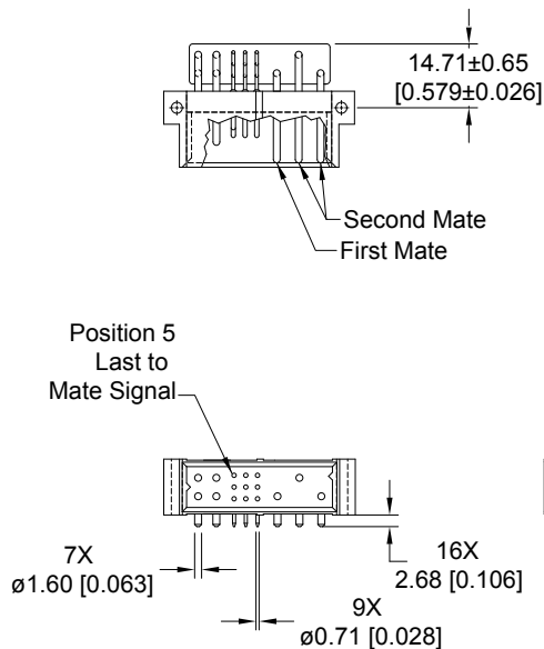
CONNECTOR DIMENSIONS
