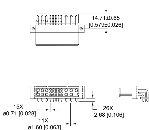
CONNECTOR DIMENSIONS
