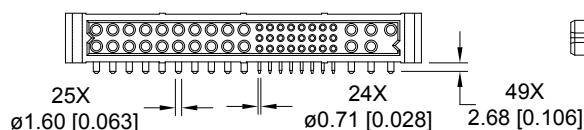
CONNECTOR DIMENSIONS
