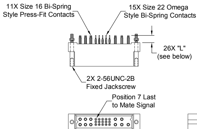
CONNECTOR DIMENSIONS
