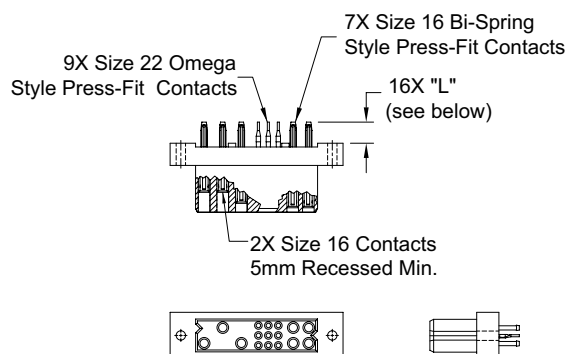
CONNECTOR DIMENSIONS
