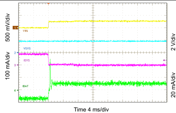
Figure 41. Exiting Battery Supplement Mode
