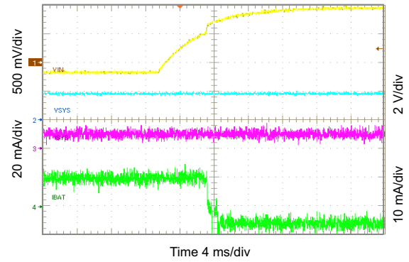
Figure 43. OVP Fault
