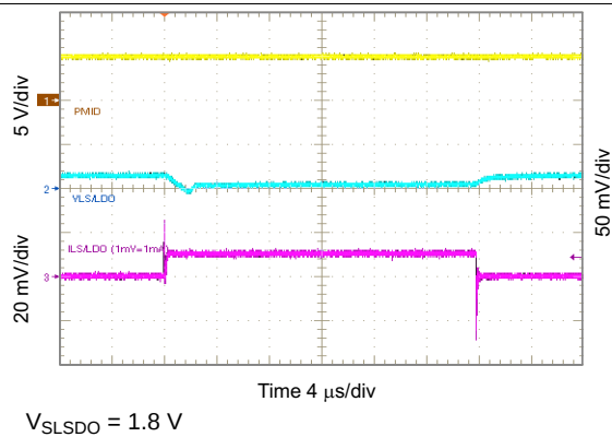
Figure 83. 1.8 V LSLDO Load Transient, 0 to 10 mA
