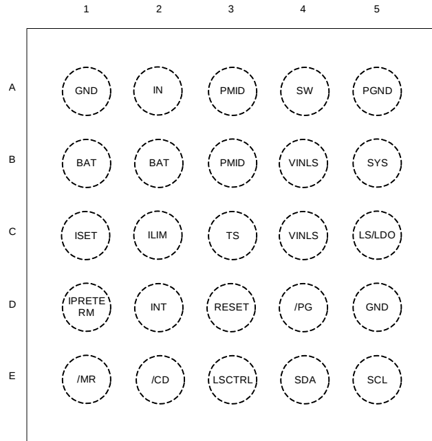
Pin Functions
