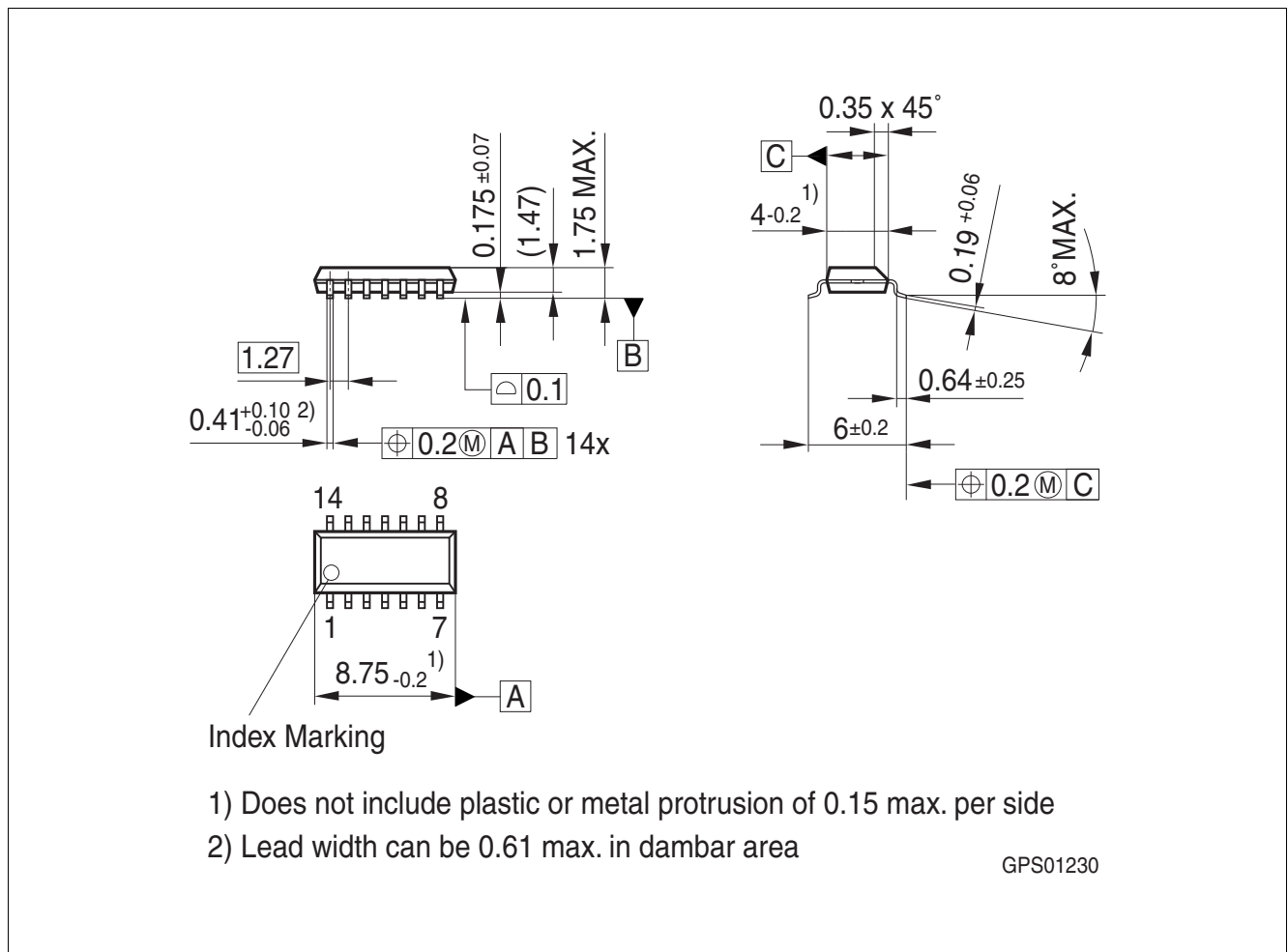
Figure 10 PG-DSO-14
