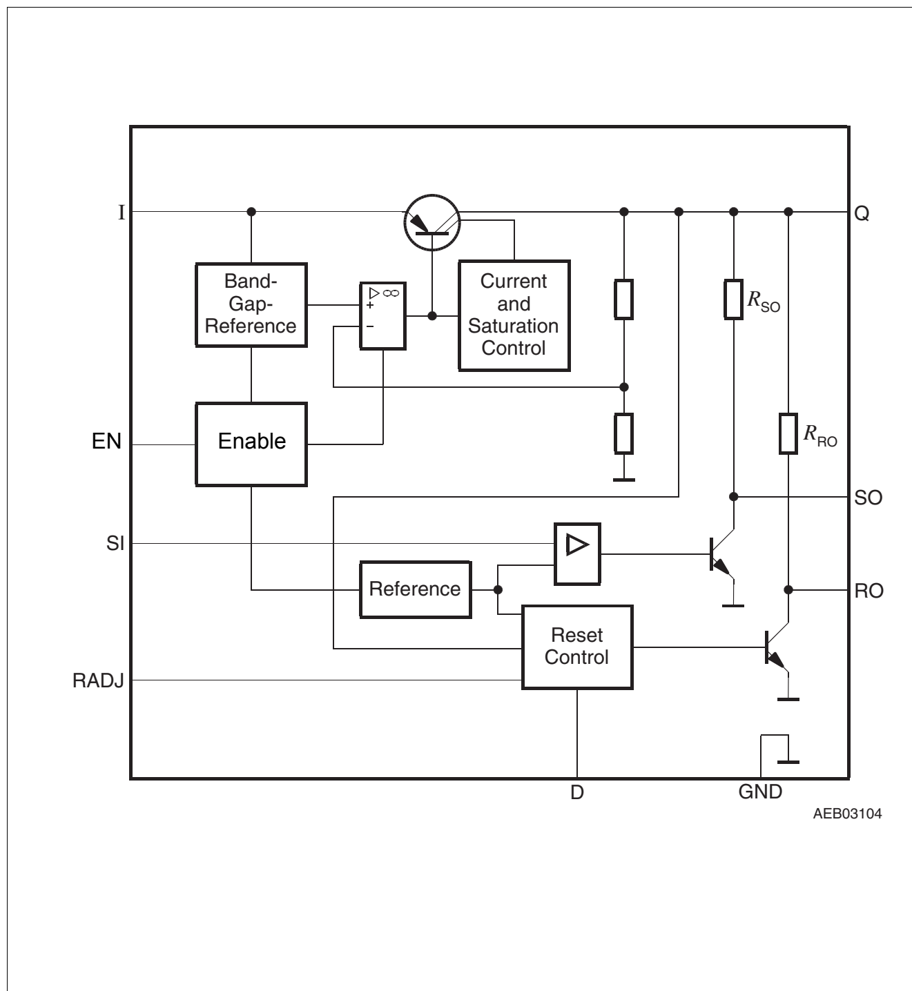
Figure 1 Block Diagram
