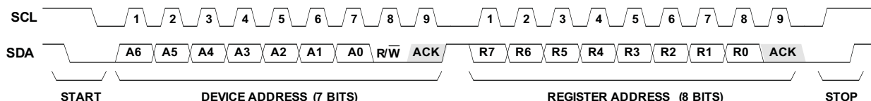
Figure 34. I 2 C Read Operation
