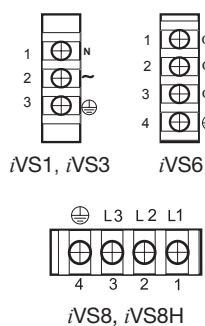
Figure 1. AC Input
