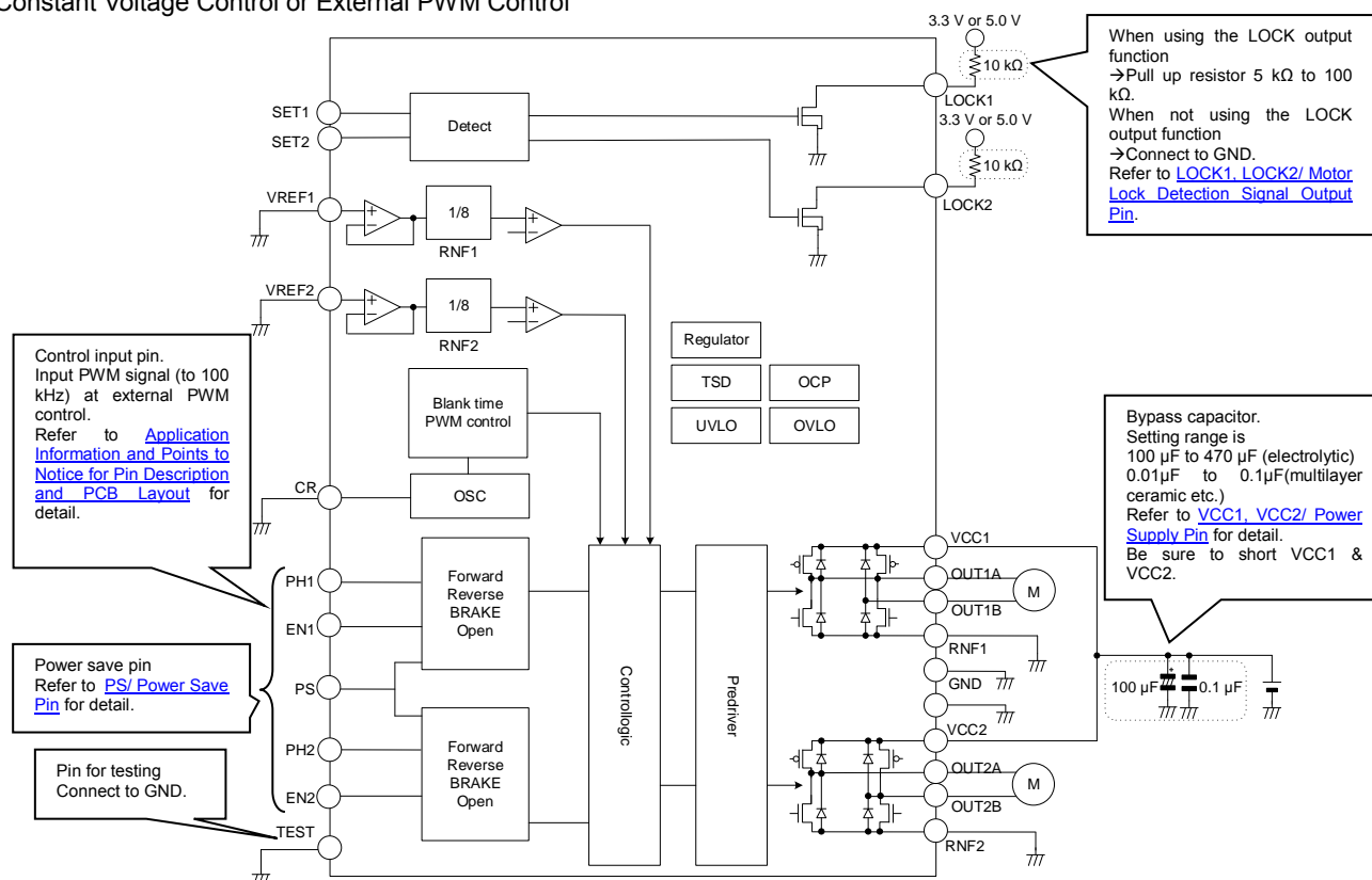
Figure 8. Block Diagram &amp; Application Circuit Diagram
