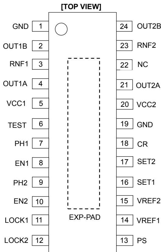
Figure 3. Pin Configuration
