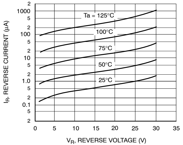
Figure 2. I_R - V_R
