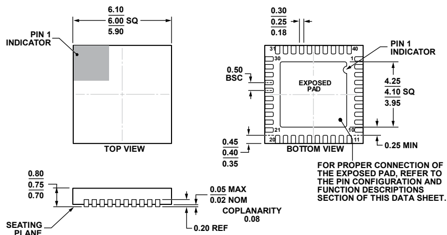
Figure 42. 40-Lead Lead Frame Chip Scale Package [LFCSP_WQ] 6 mm x 6 mm Body, Very Very Thin Quad (CP-40-9) Dimensions shown in millimeters
