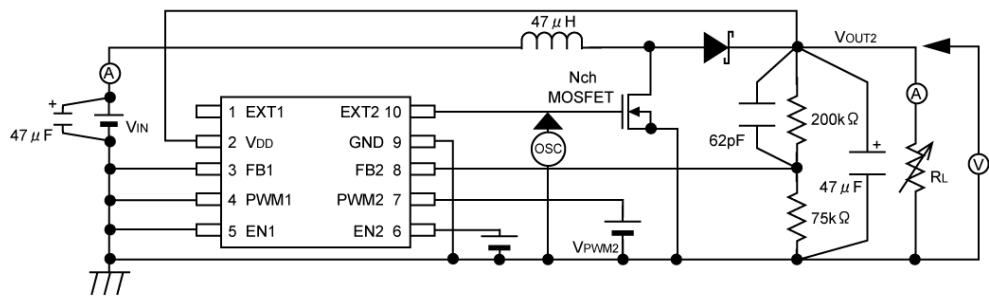
Circuit 9
