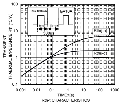
R_{\theta JA} - t CHARACTERISTICS
