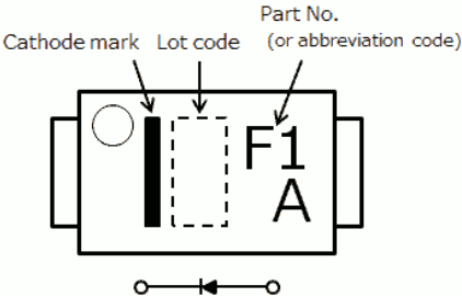
Fig. 7.1 Marking
