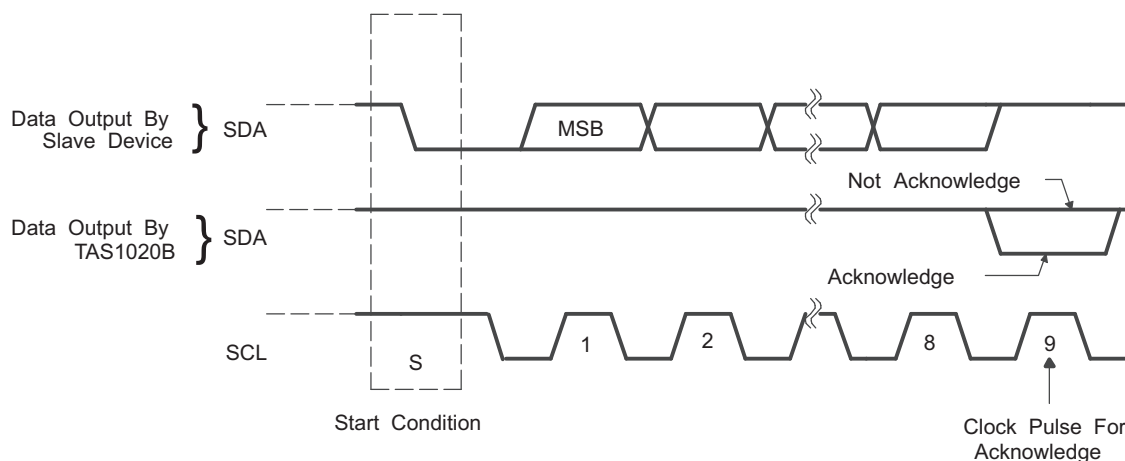
Figure 2-14. TAS1020B Acknowledge on the I²C Bus
