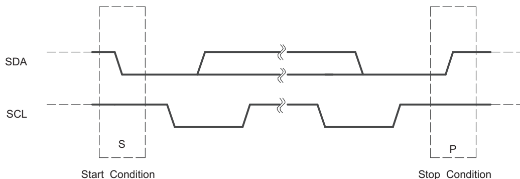
Figure 2-13. I²C START and STOP Conditions
