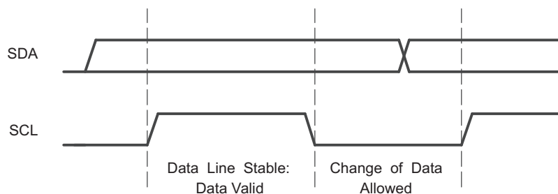
Figure 2-12. Bit Transfer on the I 2 C Bus
