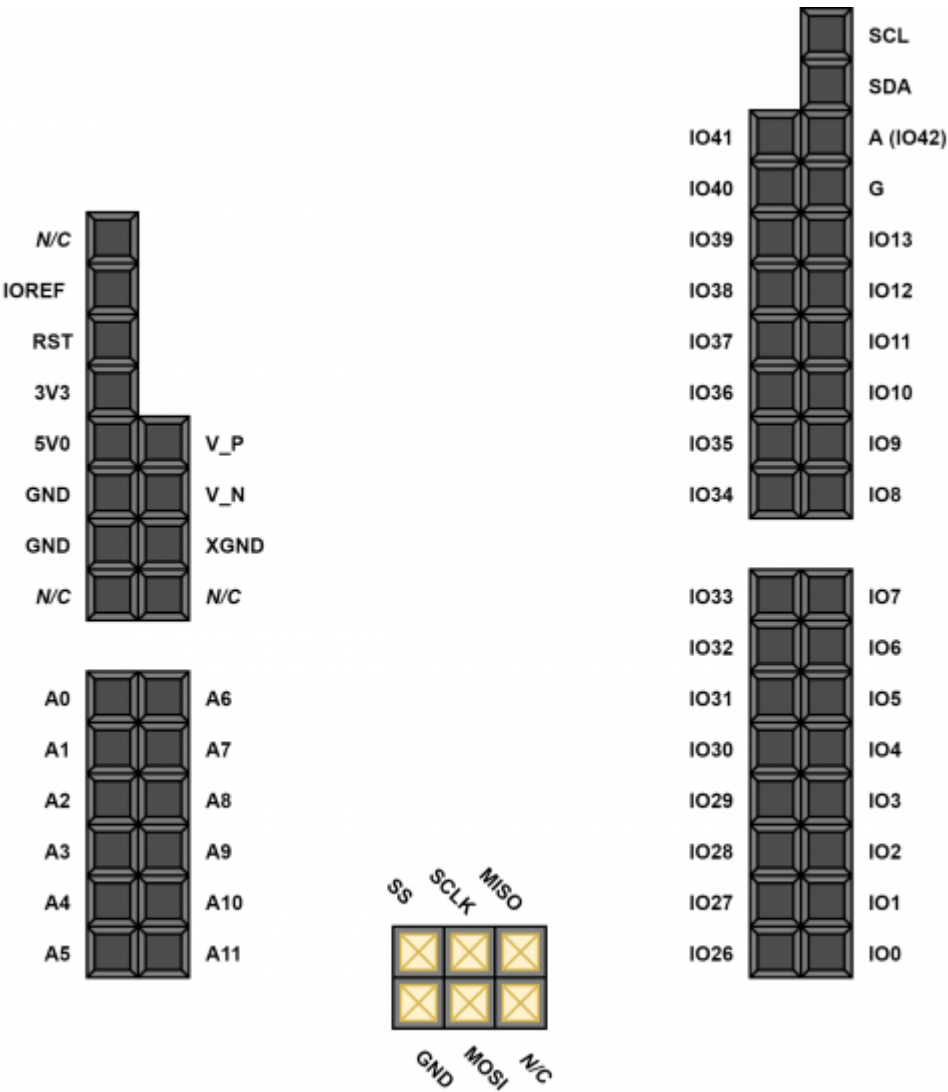
( https://reference.digilentinc.com/_media/reference/programmable-logic/cora-z7/cora-shield.png ) Figure 13.1. Shield connector pin diagram.
