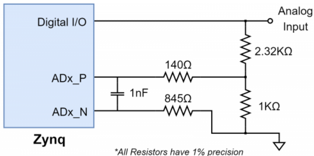
( https://reference.digilentinc.com/_media/reference/programmable-logic/cora-z7/cora-analog-single-ended.png ) Figure 13.2.1. Single-Ended Analog Inputs
