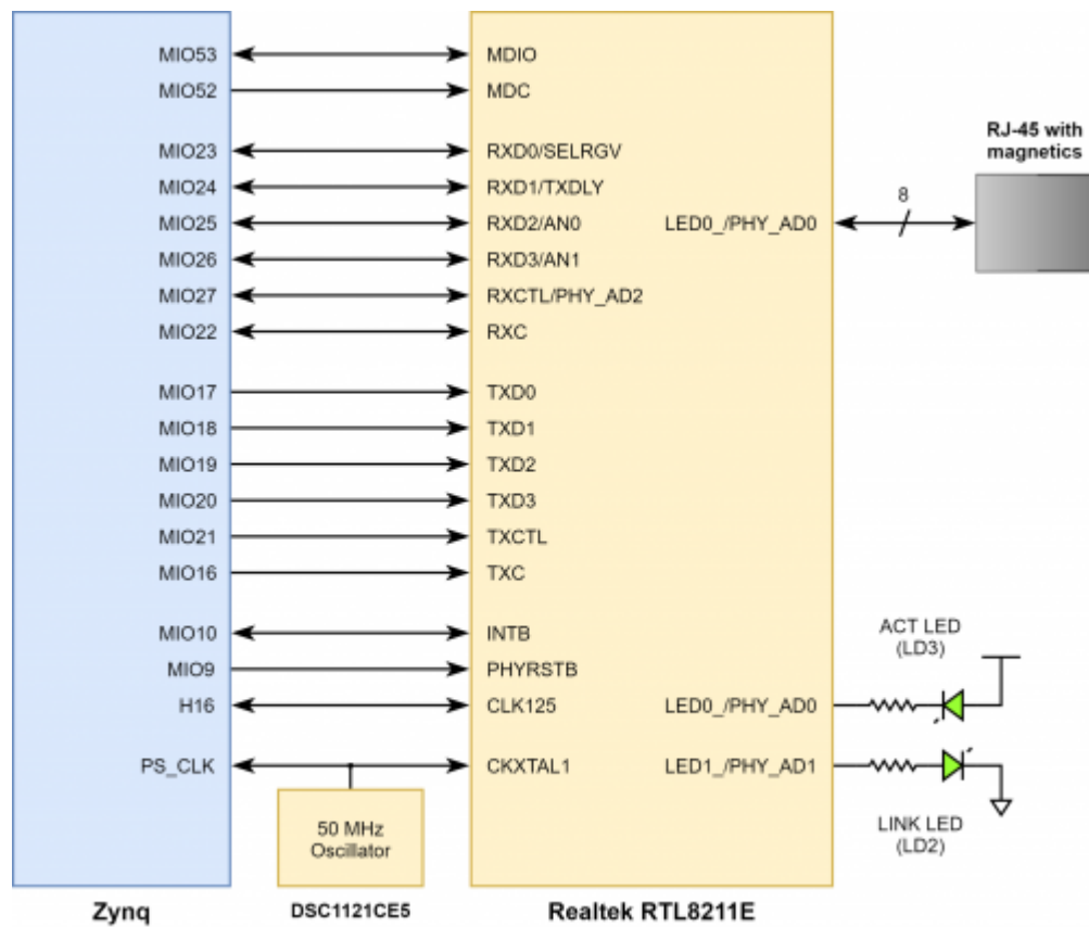
( https://reference.digilentinc.com/_media/reference/programmable-logic/cora-z7/cora-ethernet.png ) Figure 8.1. Ethernet PHY signals
