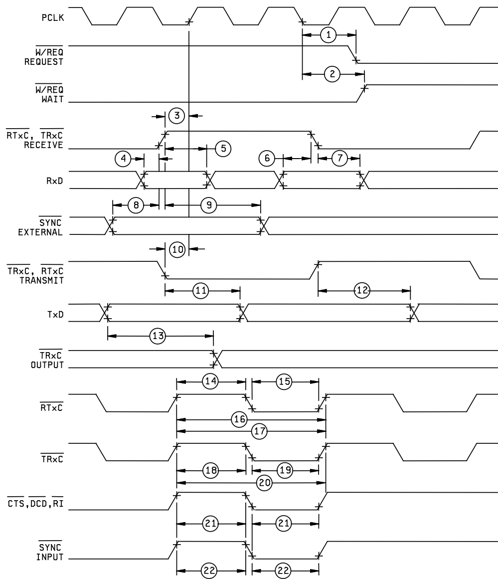
GENERAL TIMING
