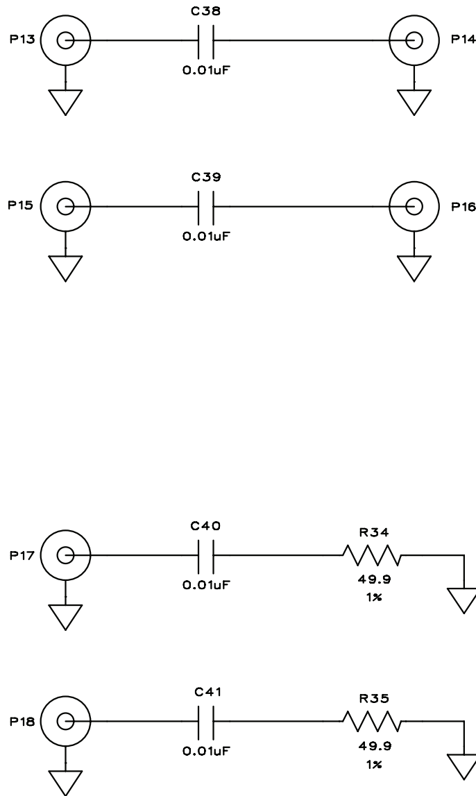
Figure 1c. MAX4986 EV Kit Schematic (Sheet 3 of 3)
