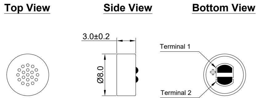
Figure 4. HBO0803A-46/1133 Mechanical Layout
