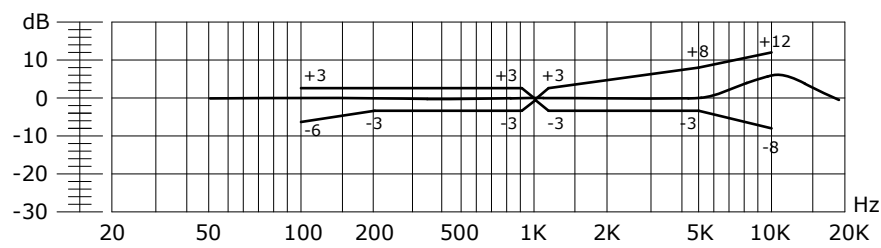
Figure 1. Frequency Response
