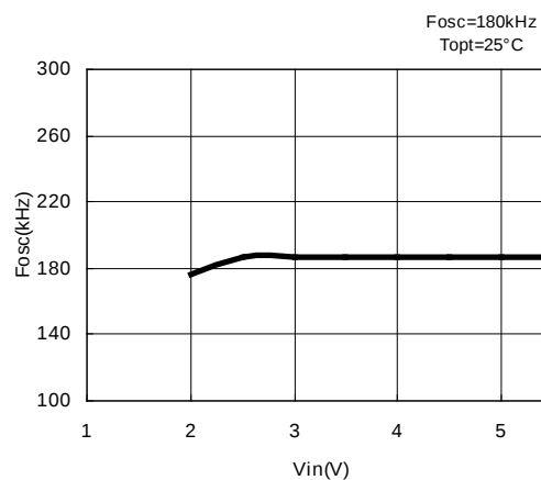
5) Osillator Frequency VS. Input Voltage R1290K102A
