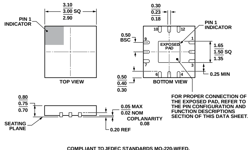
Figure 27. 12-Lead Lead Frame Chip Scale Package [LFCSP] 3 mm × 3 mm and 0.75 mm Package Height (CP-12-5) Dimensions shown in millimeters
