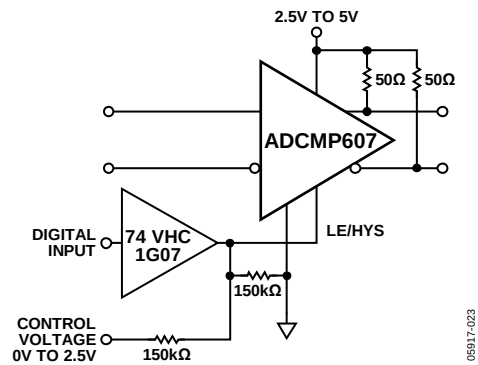
Figure 24. Hysteresis Adjustment with Latch on the ADCMP607
