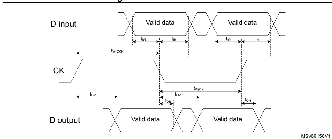
Figure 48. SDRAMC DDR mode
