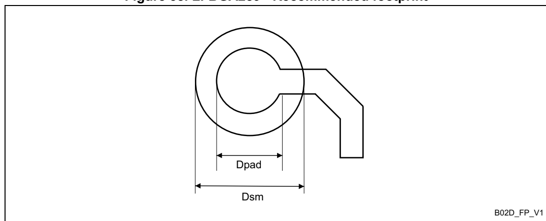
Figure 58. LFBGA289 - Recommended footprint
