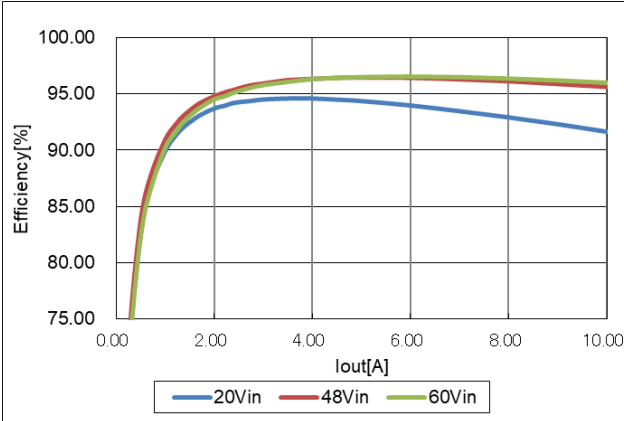
Figure 4. Efficiency (Linear scale)
