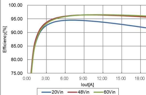
Figure 12. Efficiency (Linear scale)
