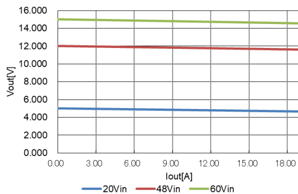
Figure 14. Output voltage
