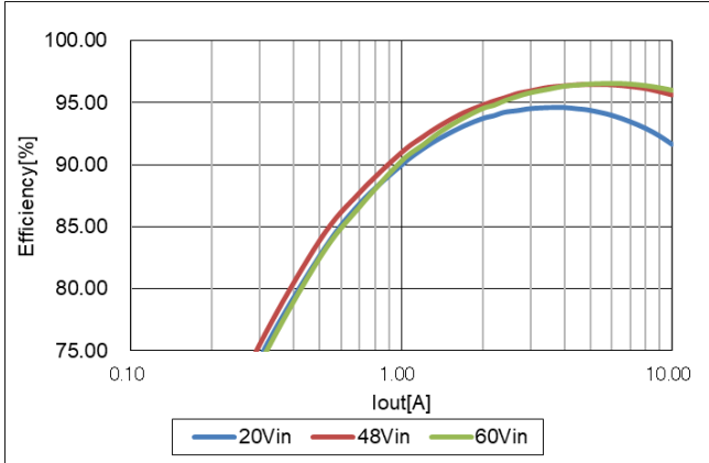
Figure 5. Efficiency (Log scale)
