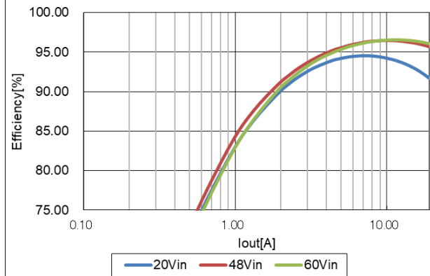
Figure 13. Efficiency (Log scale)
