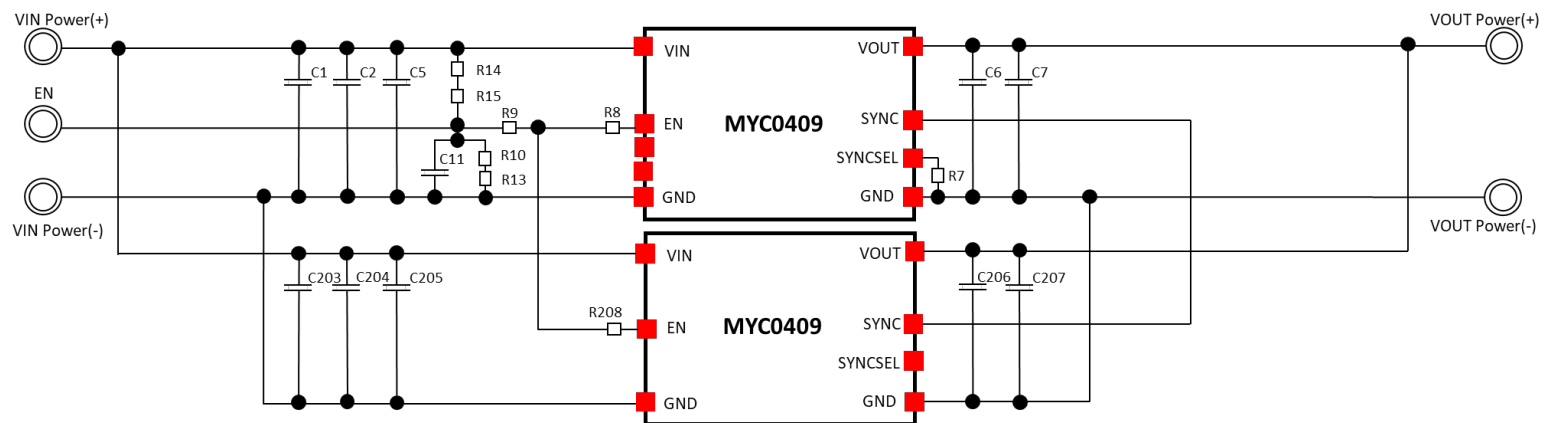
Figure 20. MYC0409-NA-120WD-EVM schematic
