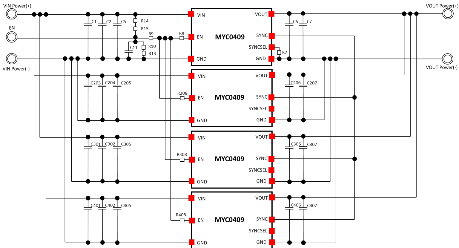
Figure 21. MYC0409-NA-200WD-EVM schematic
