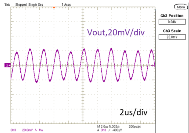
(V OUT =12V, I OUT =12A, T a =25degC) Figure 7. VOUT ripple Waveform
