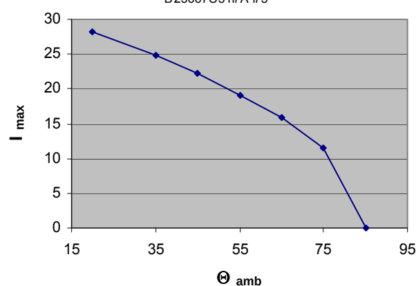
Max. allowable current (rms) at specific ambient Temp. B25667C5117A 175
