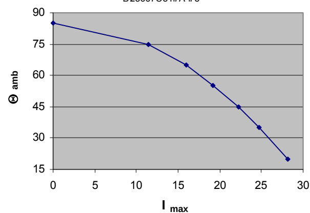
Max. allowable ambient Temp. at specific current (rms) B25667C5117A 175
