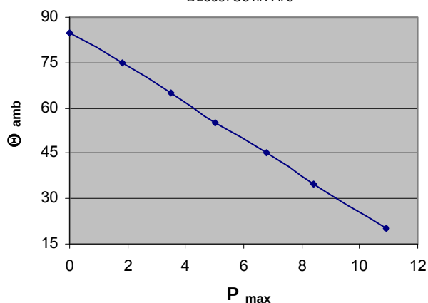
Max. allowable ambient Temp. at specific power loss B25667C5117A 175
