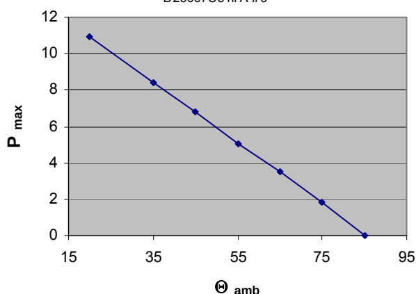
Max. allowable power loss at specific ambient Temp. B25667C5117A 175
