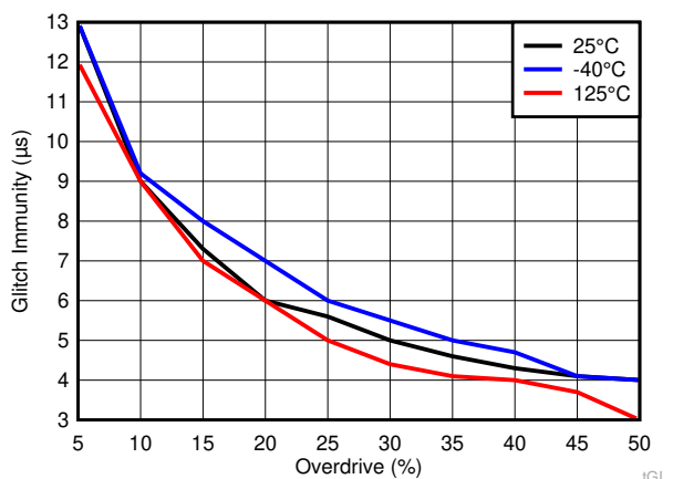
Figure 7-26. Glitch Immunity Versus Overdrive for TLV803EA29
