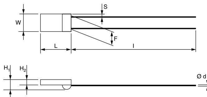
DIMENSIONS - PTL sensor type, relevant physical dimensions
