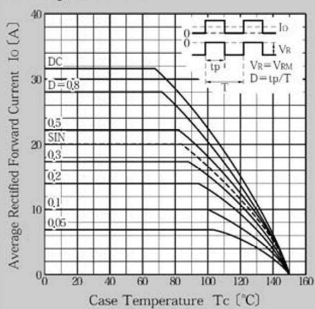
Derating Curve T_c - I_o
