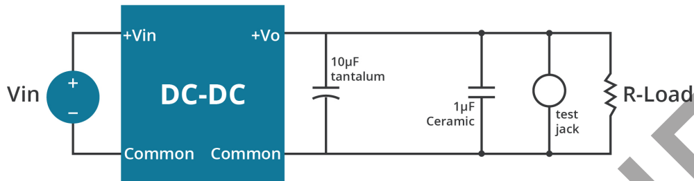
Figure 9 Output Voltage Ripple and Noise Measurement Set-up
