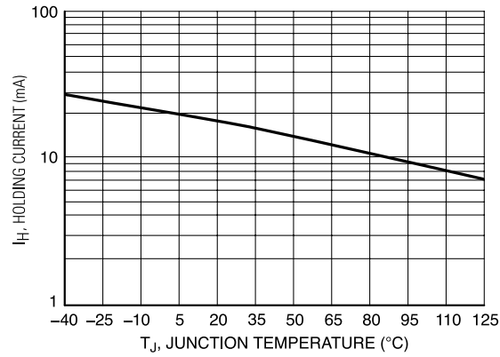
Figure 5. Typical Holding Current vs Junction Temp
