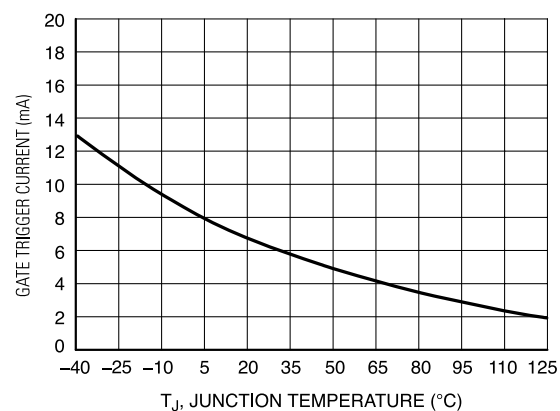
Figure 4. Typical Gate Trigger Current vs Junction Temp
