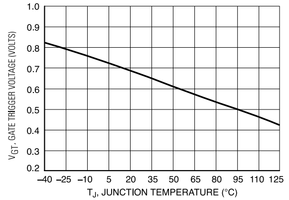
Figure 6. Typical Gate Trigger Voltage vs Junction Temp
