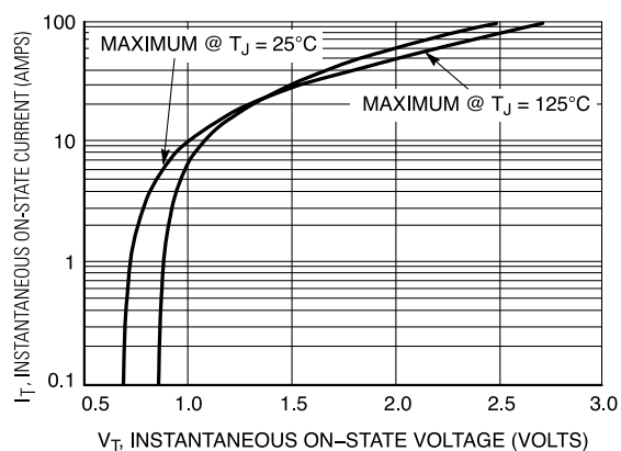
Figure 3. Typical On-State Characteristics
