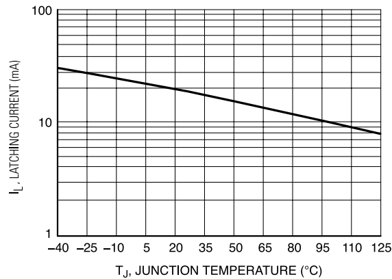
Figure 7. Typical Latching Current vs Junction Temp
