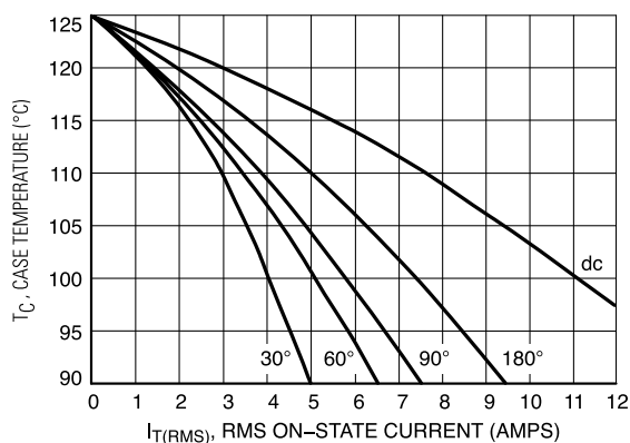
Figure 1. Typical RMS Current Derating
