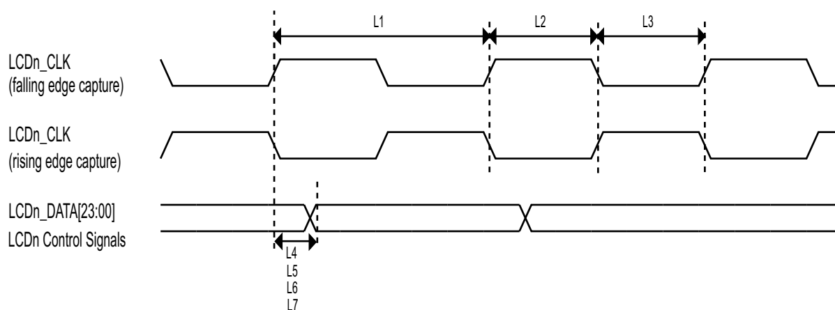
Figure 43. LCD Timing
