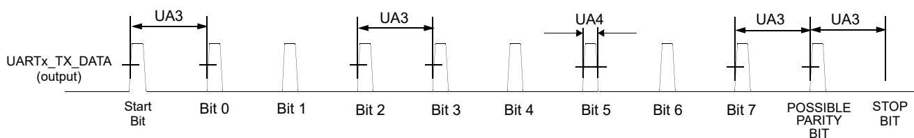
Figure 57. UART IrDA Mode Transmit Timing Diagram
