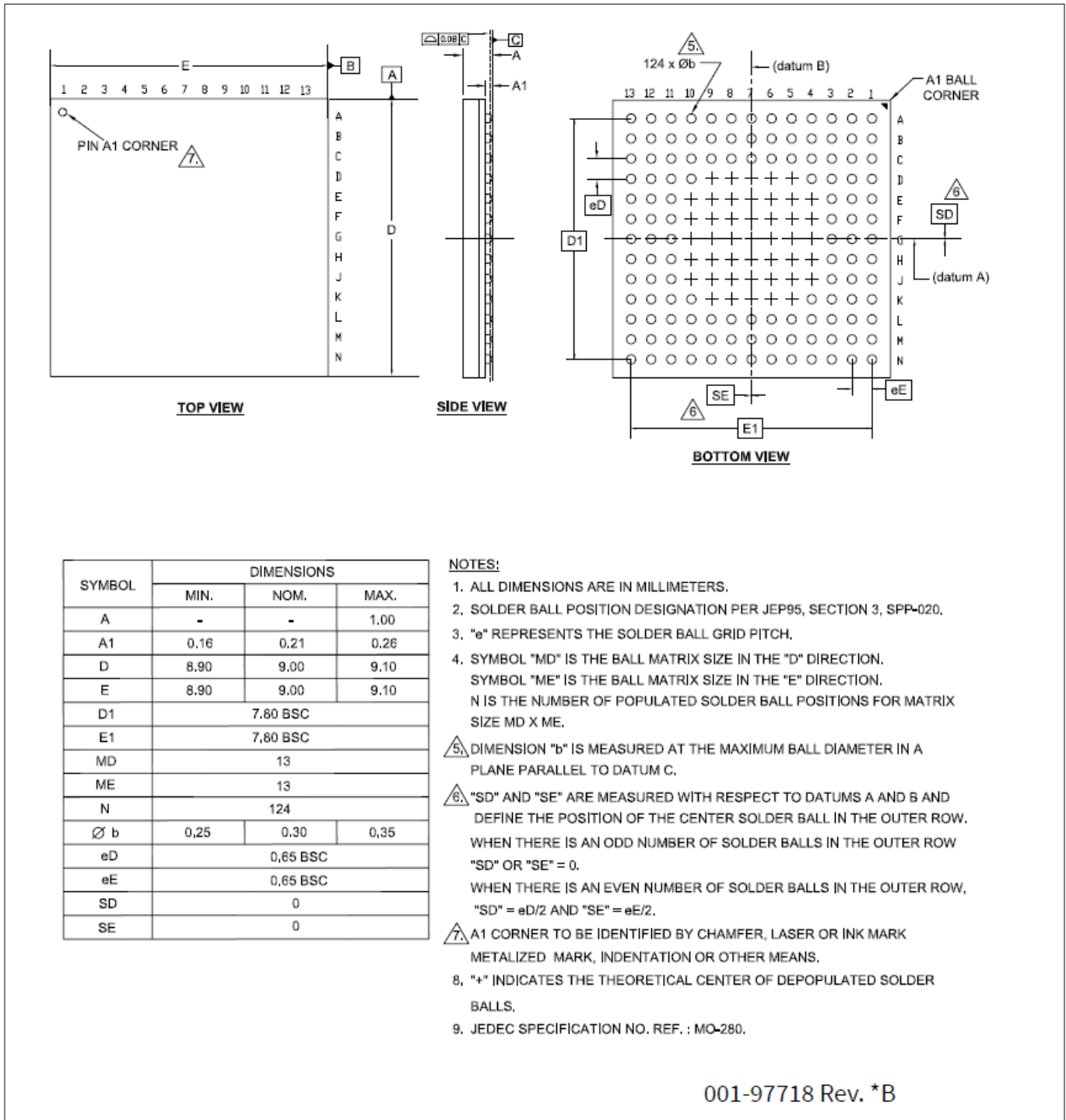
Figure 21 124-ball VFBGA (9.0 x 9.0 x 1.0 mm) BZ0AA/VZC124/D2A124 package outline (PG-VFBGA-124)
