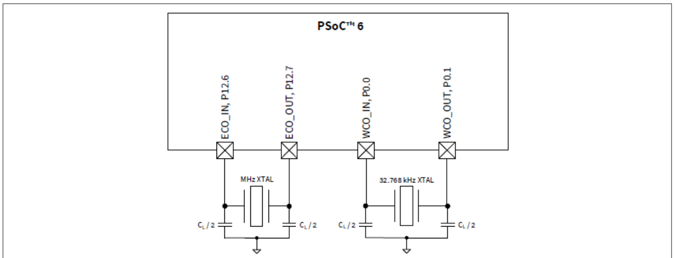
Figure 4 Oscillator circuits
