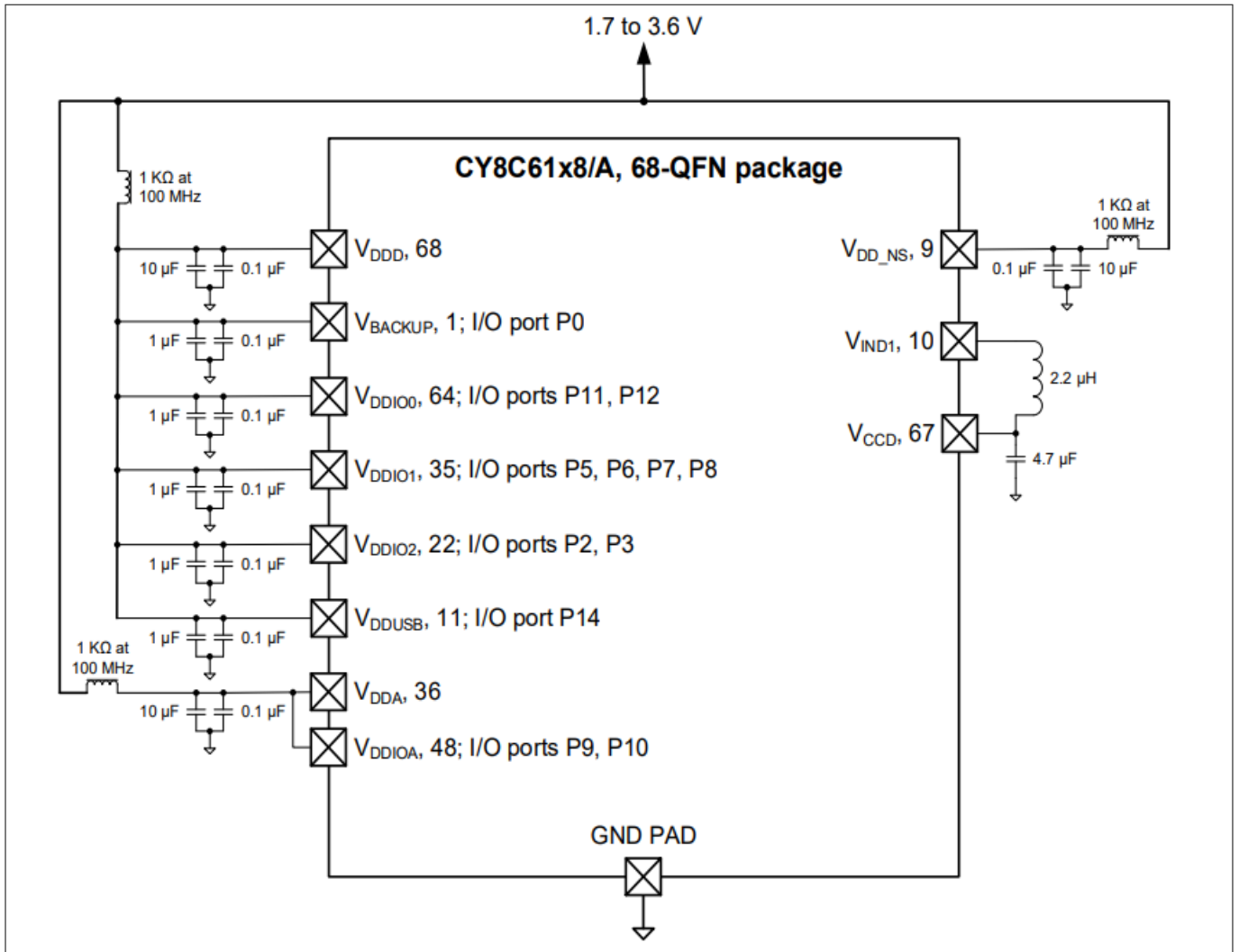
Figure 17 68-QFN Power connection diagram
