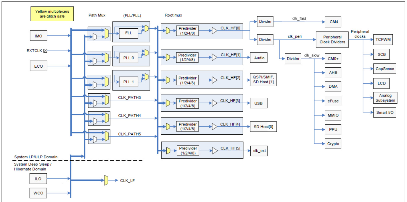
Figure 3 Clocking diagram
