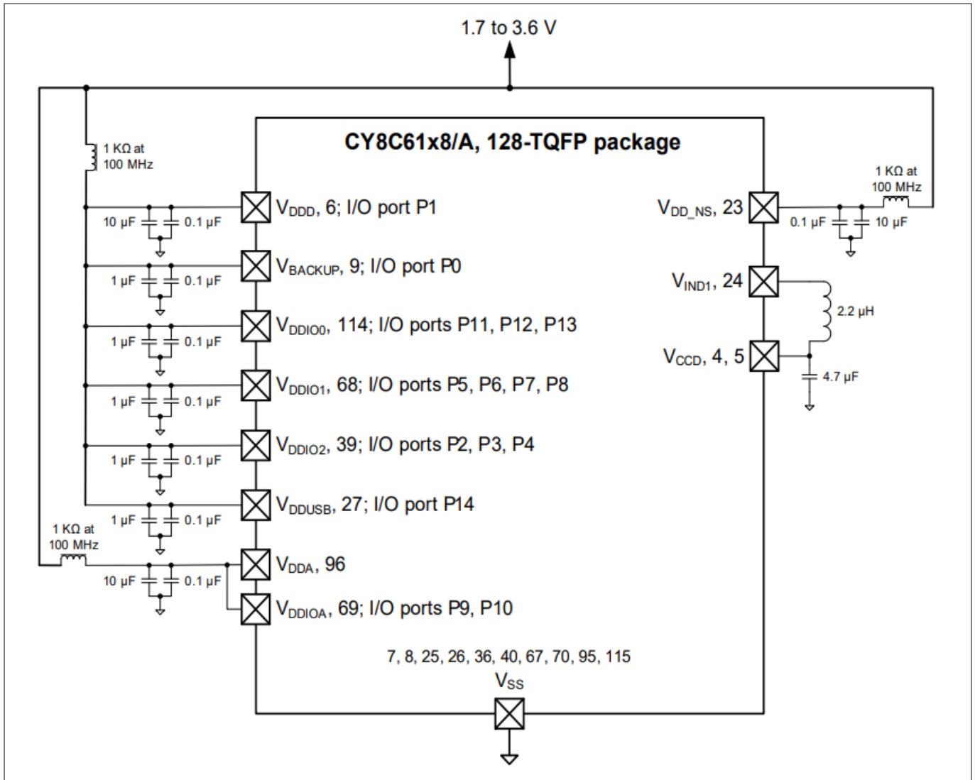
Figure 11 128-TQFP Power connection diagram
