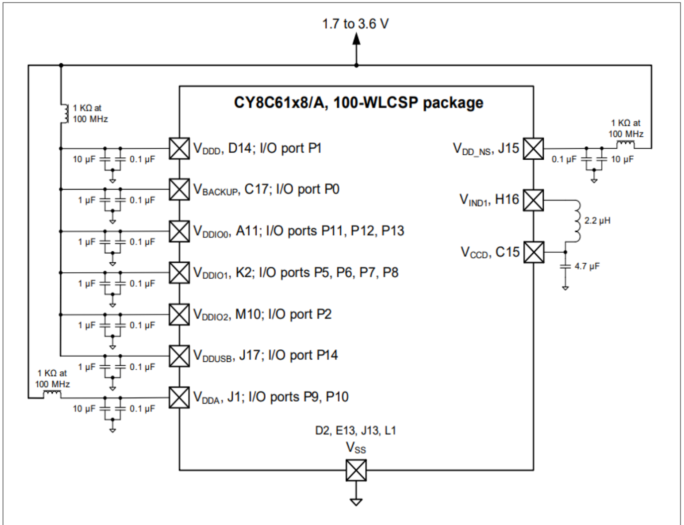
Figure 15 100-WLCSP Power connection diagram
