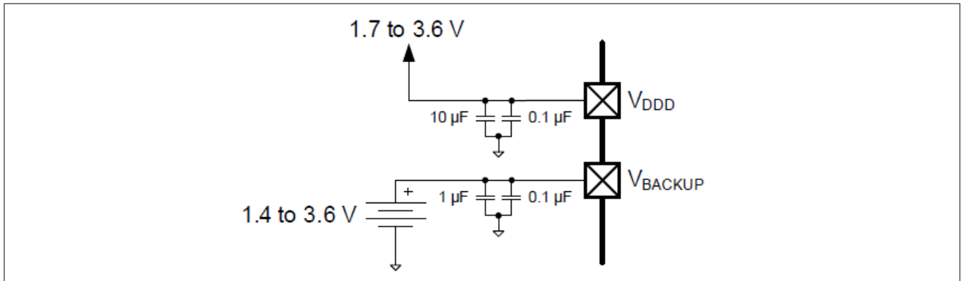
Figure 19 Separate battery connection to V_{BACKUP}
