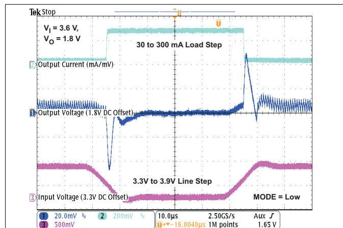
Figure 29. Combined Line/Load Transient Response
