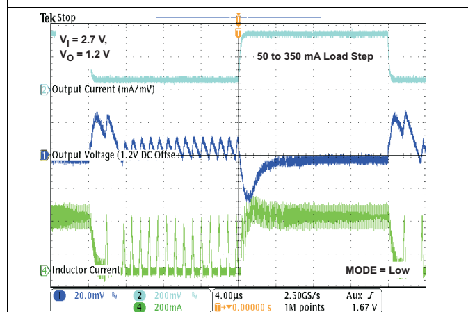
Figure 33. Load Transient Response in PFM/PWM Operation
