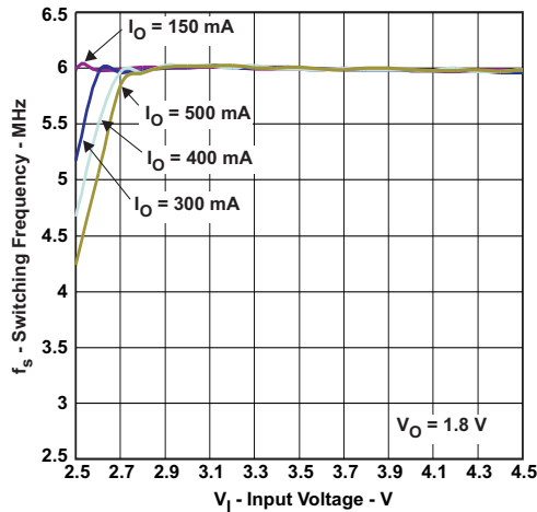
Figure 13. PFM/PWM Boundaries
