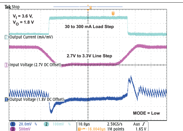
Figure 30. Combined Line/Load Transient Response
