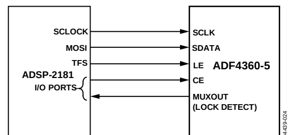
Figure 20. ADSP-2181 to ADF4360-5 Interface
