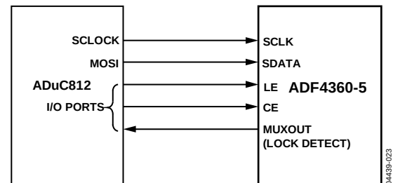
Figure 19. ADuC812 to ADF4360-5 Interface
