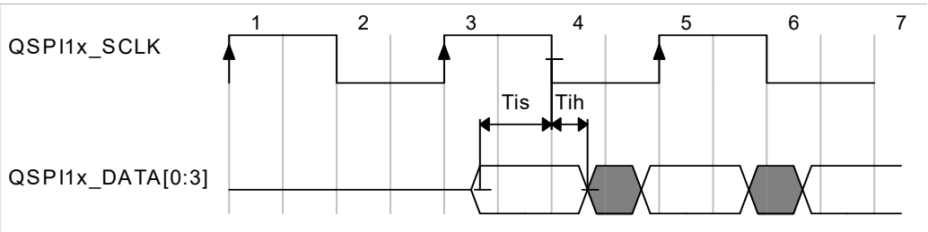
Figure 55. QuadSPI Input/Read Timing (SDR mode with internal sampling)
