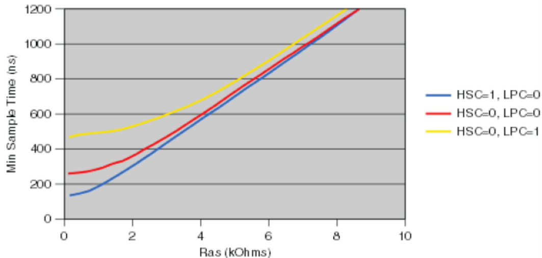
Figure 82. Minimum Sample Time versus Ras (Cas = 10pF)
