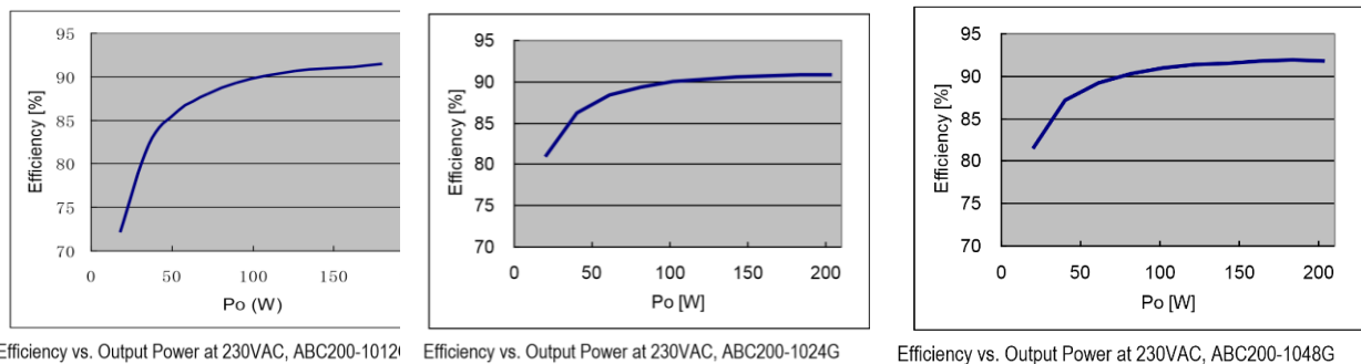
Figure 4. Efficiency Curves
