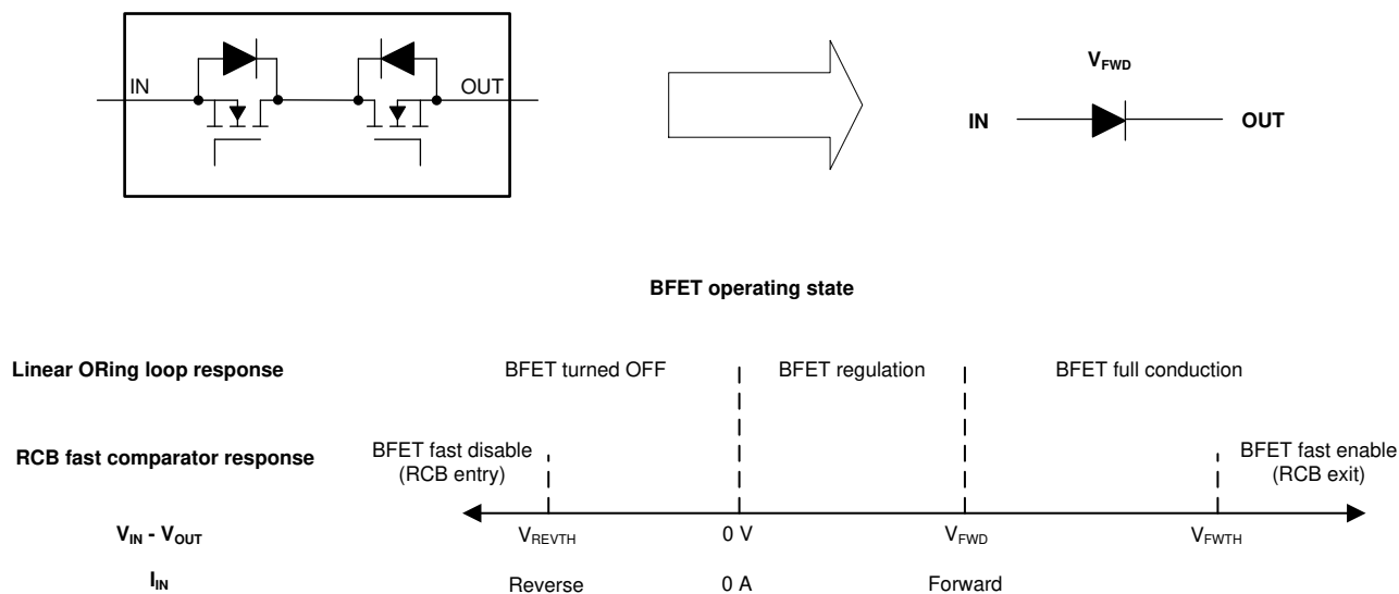
Figure 8-13. Reverse Current Blocking Response
