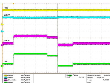
Figure 8-12. Analog Load Current Monitor Response
