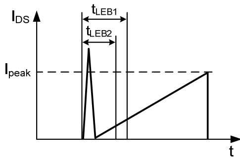
Figure 4: Leading-Edge Blanking
