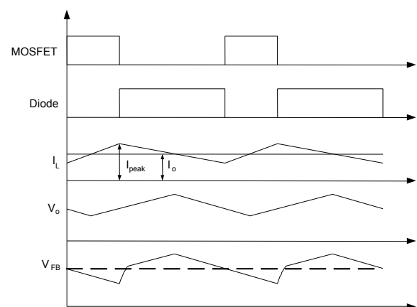
Figure 3: Constant-Voltage Regulation
