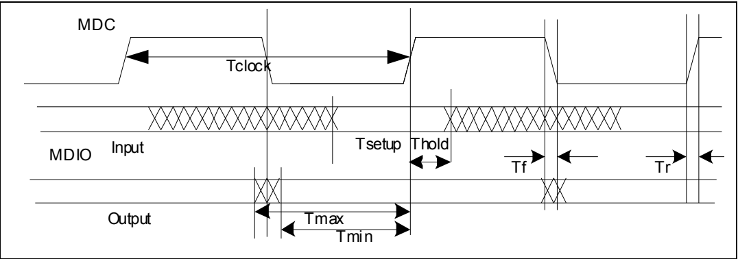
Figure 39. MDC waveforms
