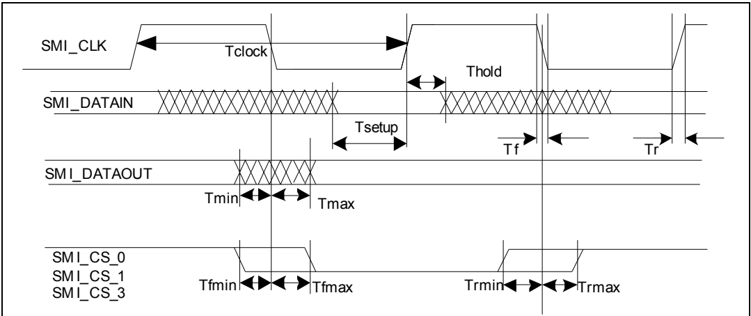
Figure 41. SMI waveforms
