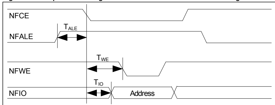
Figure 27. In/out data address signal waveforms for 8-bit NAND Flash configuration
