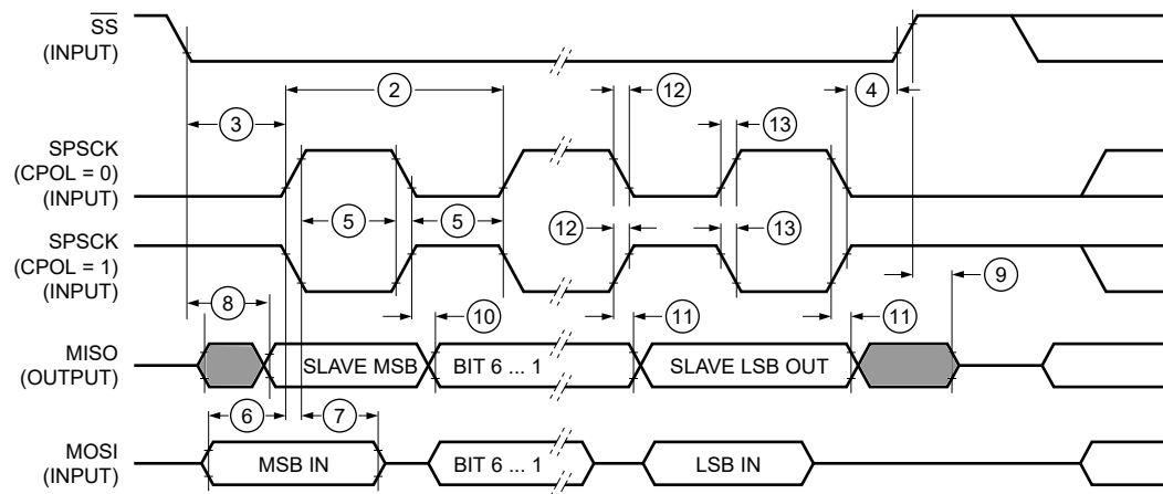
Figure 18. LPSPI Slave Mode Timing (CPHA=0)
