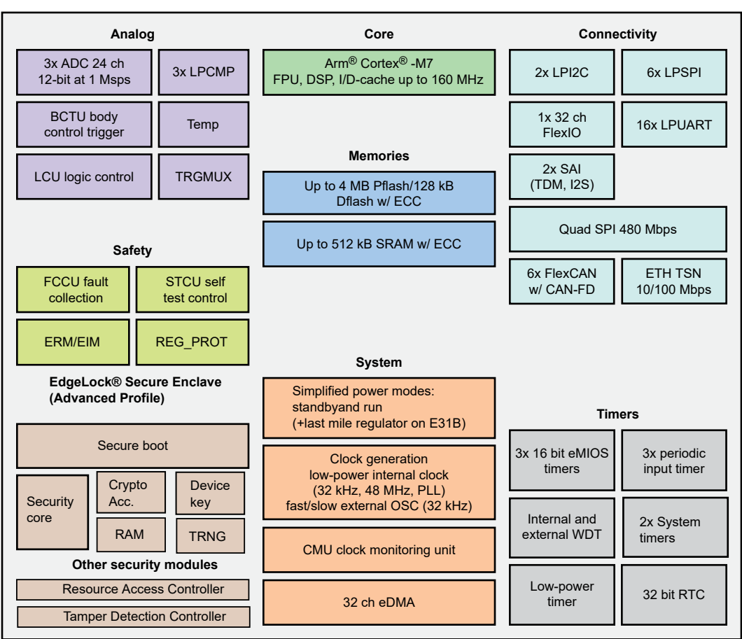
Figure 1. MCX E31 product series block diagram MCU
