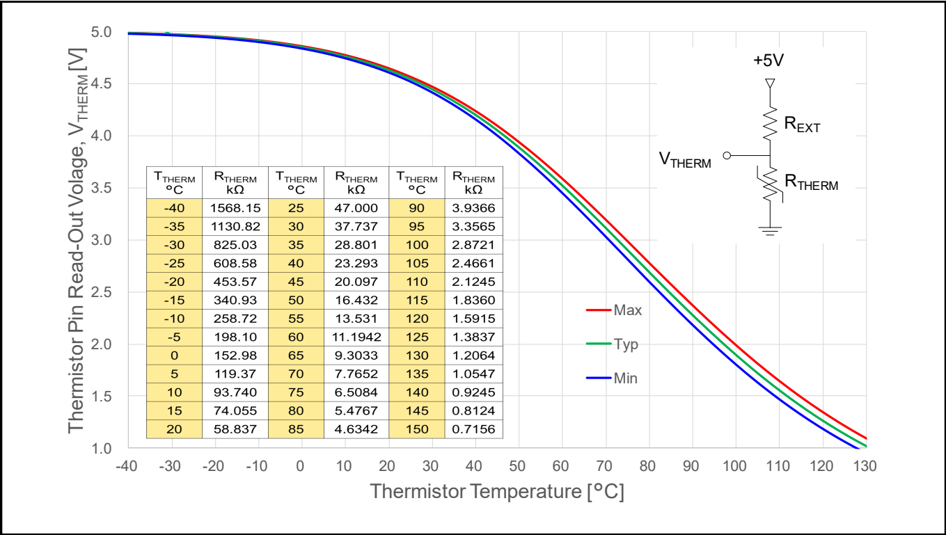
Figure 7 Thermistor readout vs. temperature (with 4.7kohm R EXT pull-up resistor) and typical thermistor resistance values vs. temperature table (For more details, please refer to the application note ‘AN2018-13 CIPOS™ IM393-XX IPM technical description_1R0_final’)
