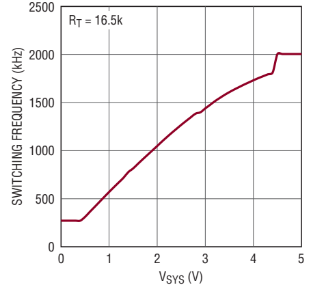
Switching Frequency vs V_{\text{SYS}}
