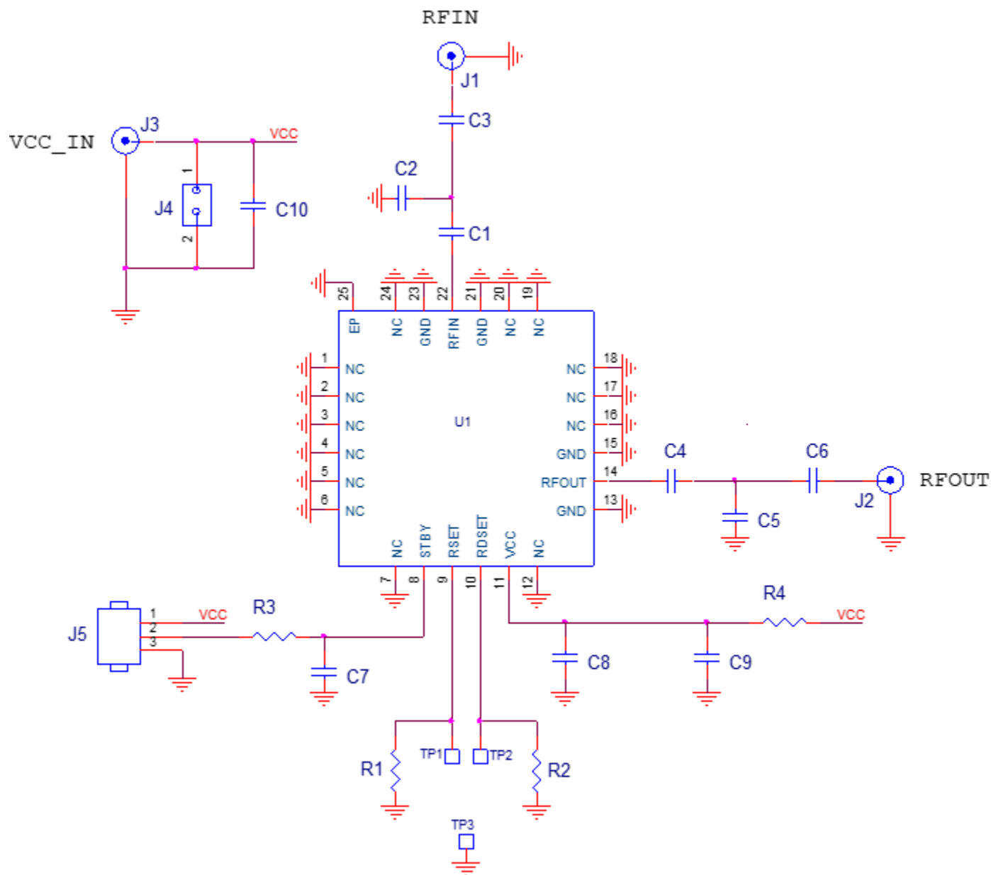
Figure 17. Electrical Schematic
