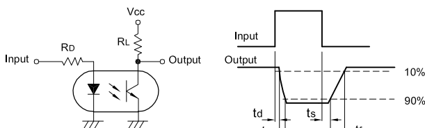
Test Circuit for Response Time
