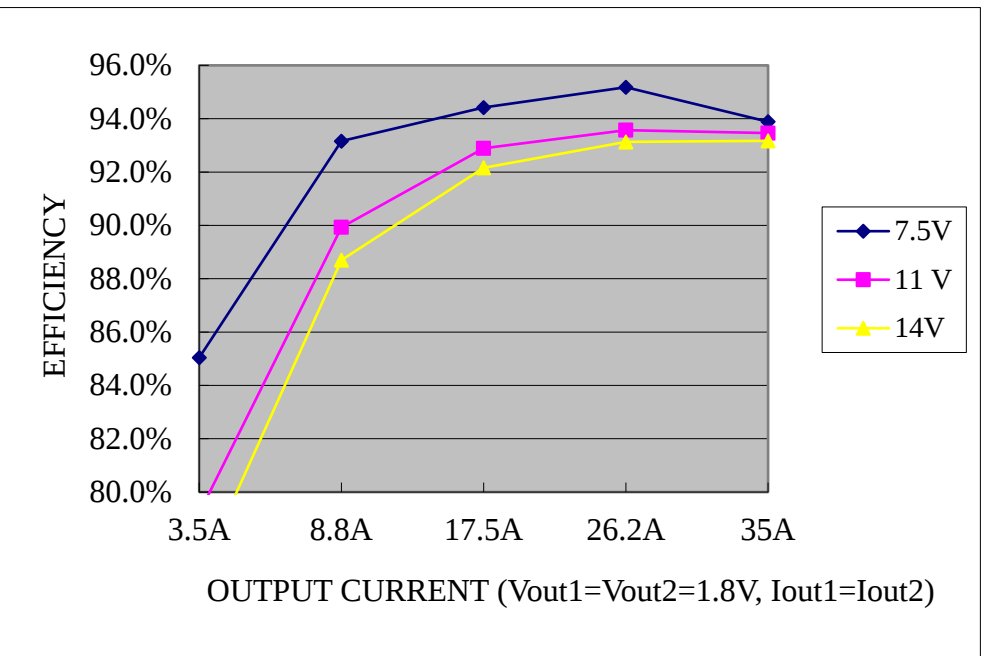
Figure 2. Efficiency data-2
