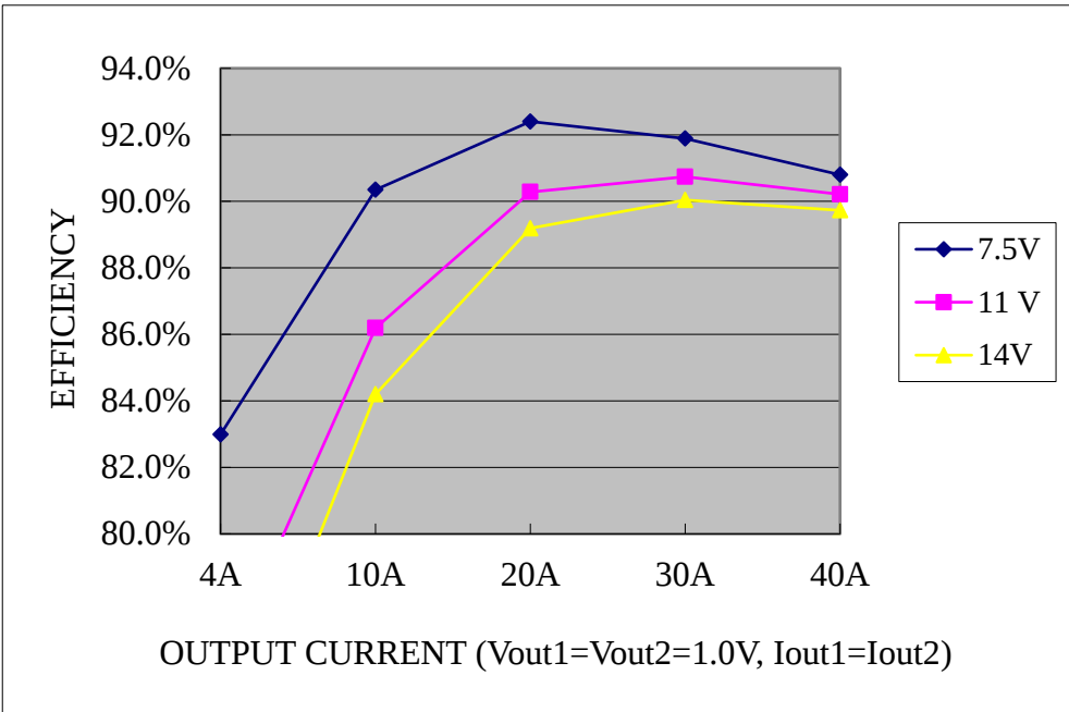
Figure 1. Efficiency data-1
