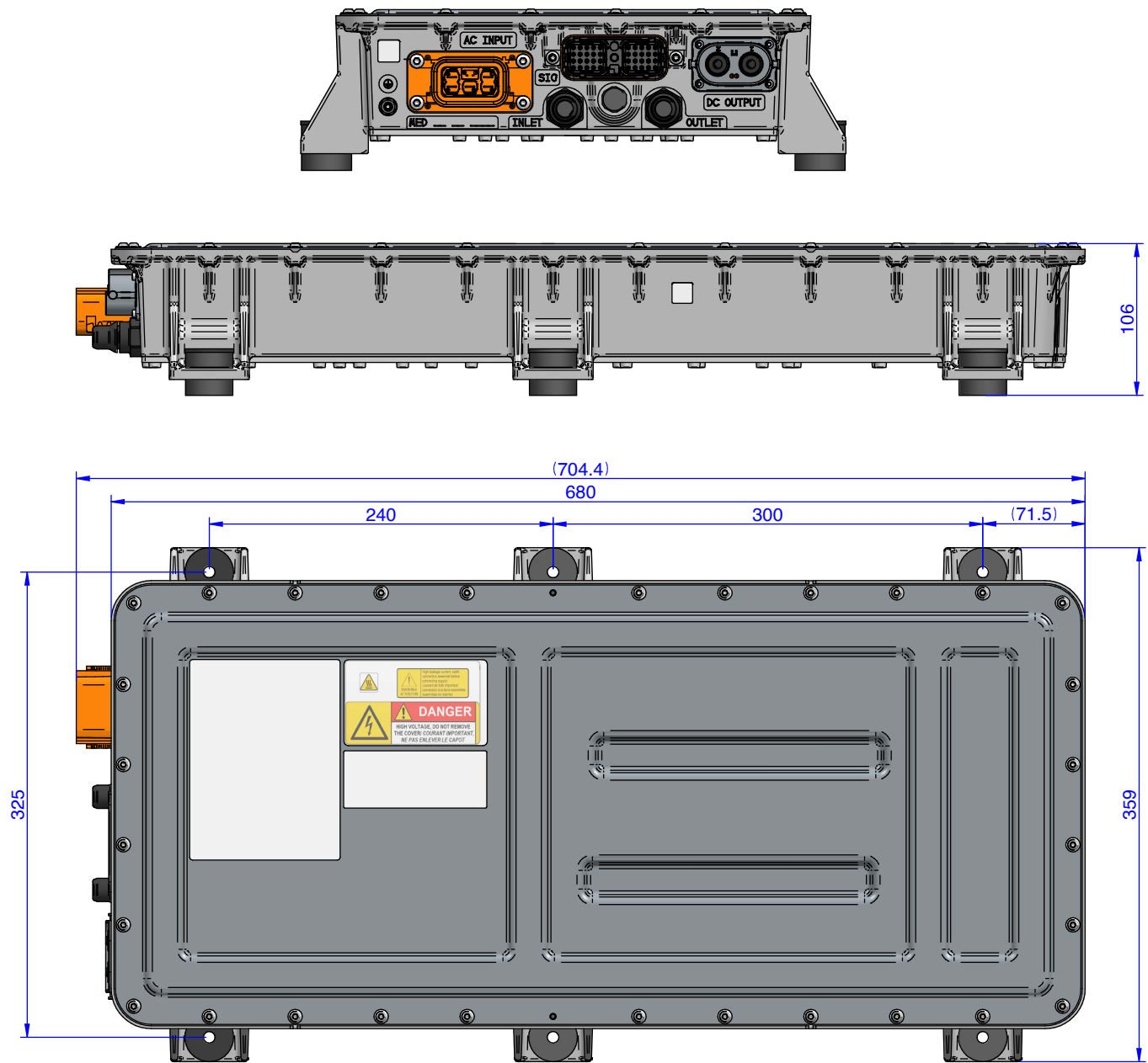
Figure 1. Mechanical Dimensions
